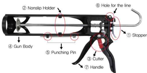
Silicone Gun
